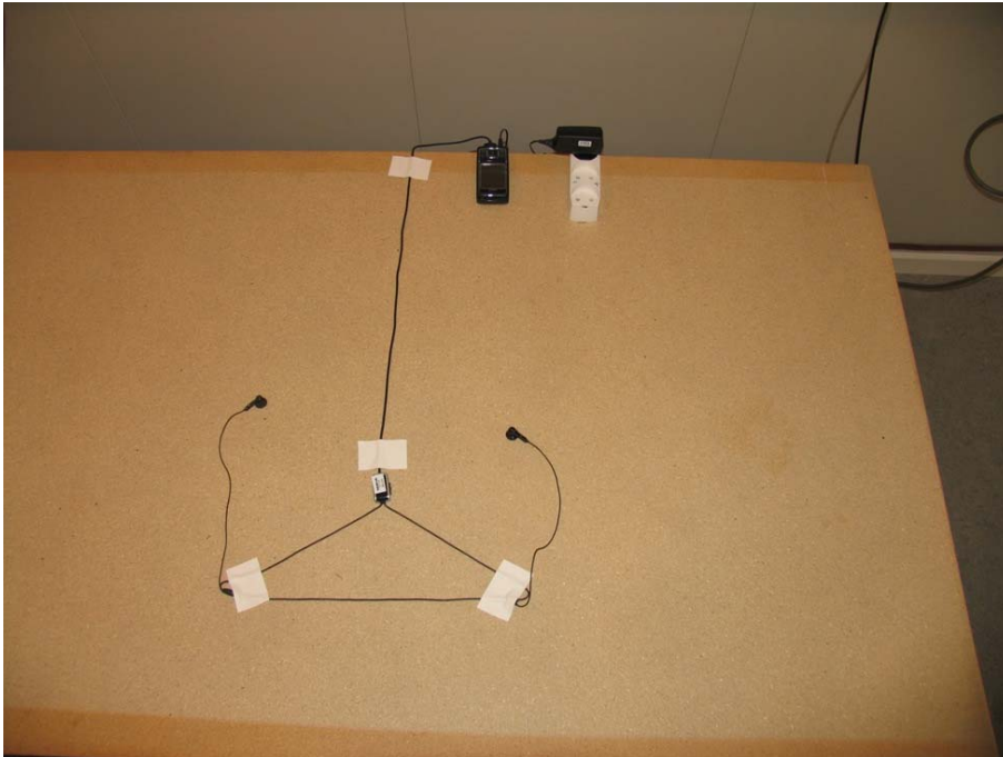
Picture 3 AC powerline conducted emission measurement
