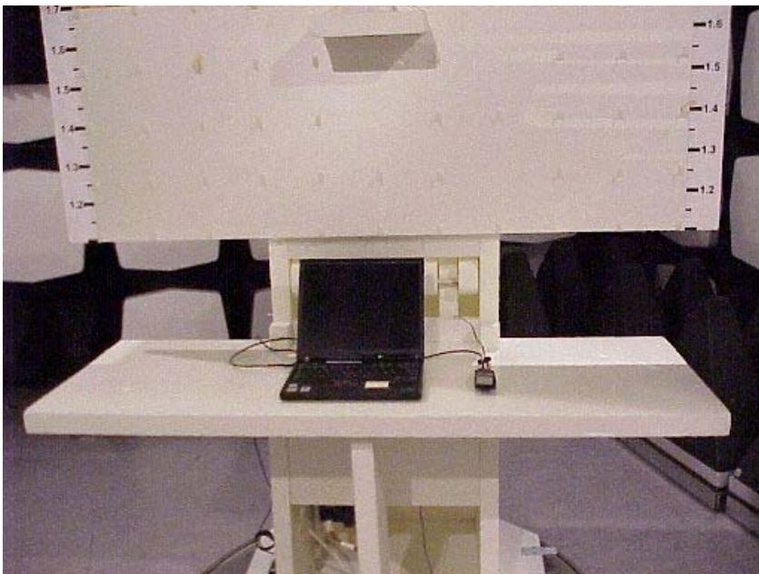
Picture 2 Radiated emission measurement GSM1900 RX and BT TX + Computer peripherals
