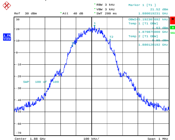
GSM mode, channel 661 / 1880.0 MHz
