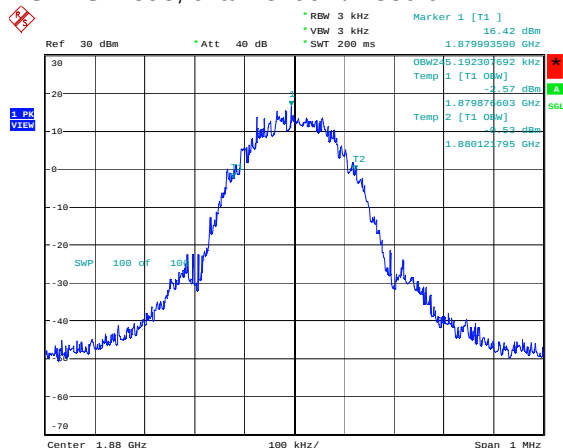
EGPRS mode, channel 661 / 1880.0 MHz
