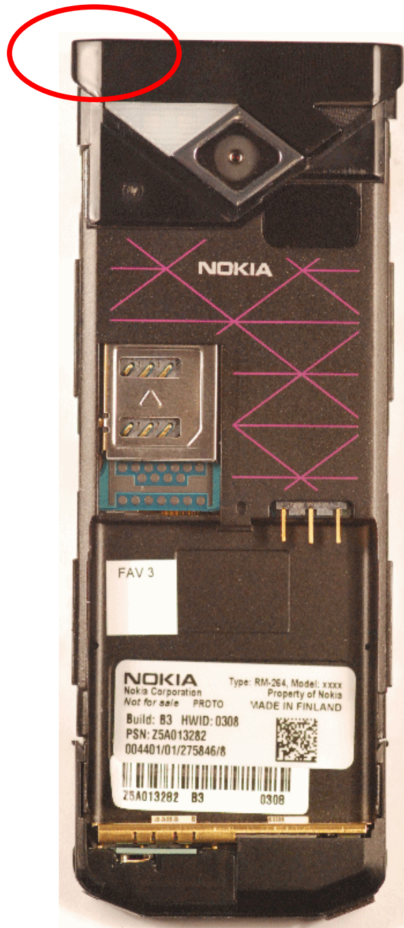
BT antenna
