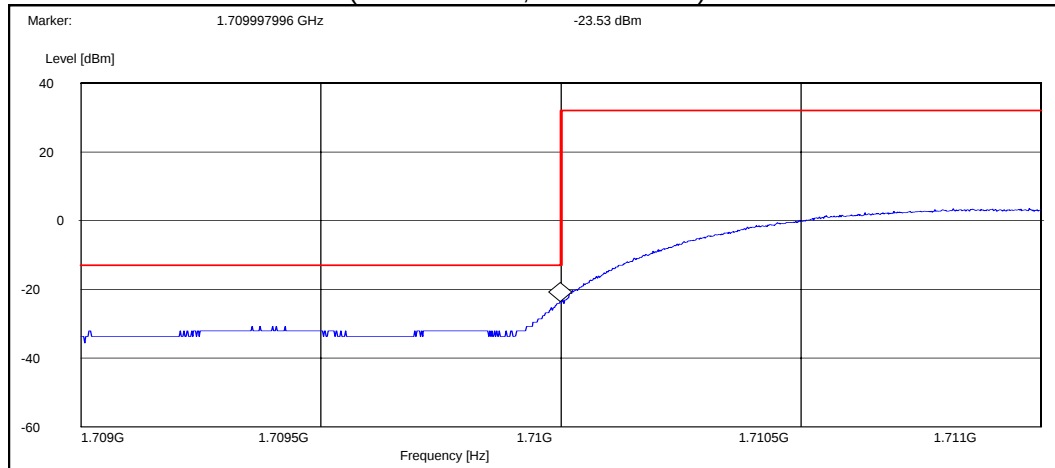
Channel 1312 / 1712.4 MHz (Peak detector, RBW: 50 kHz)
