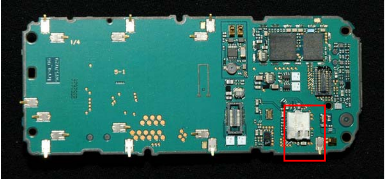
LCD Side (BOT side in parts list). Area marked in Red is BT transceiver module.
