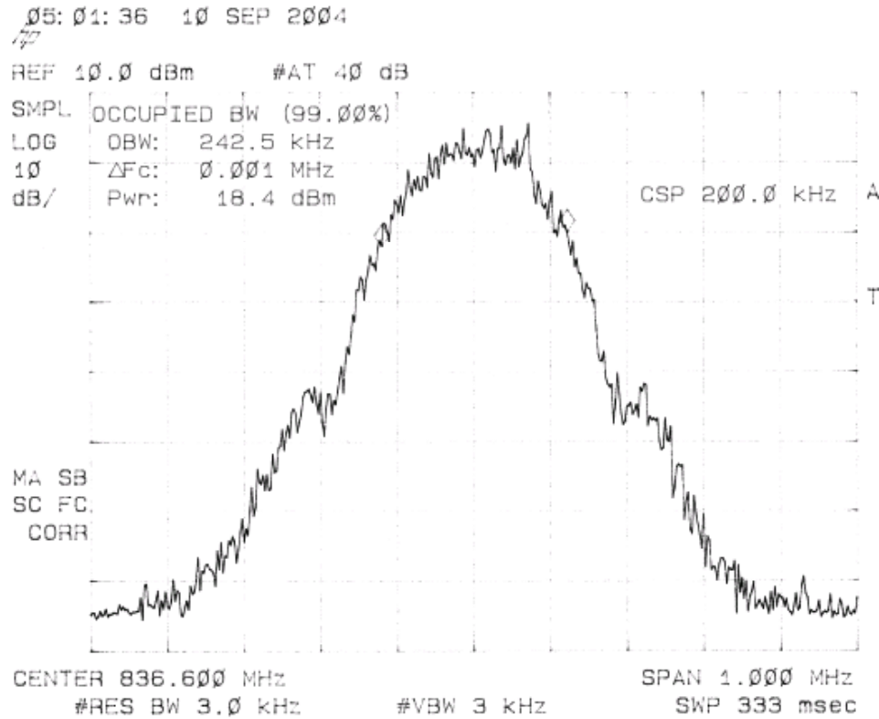
Picture 4. 99% occupied bandwidth, channel 190
