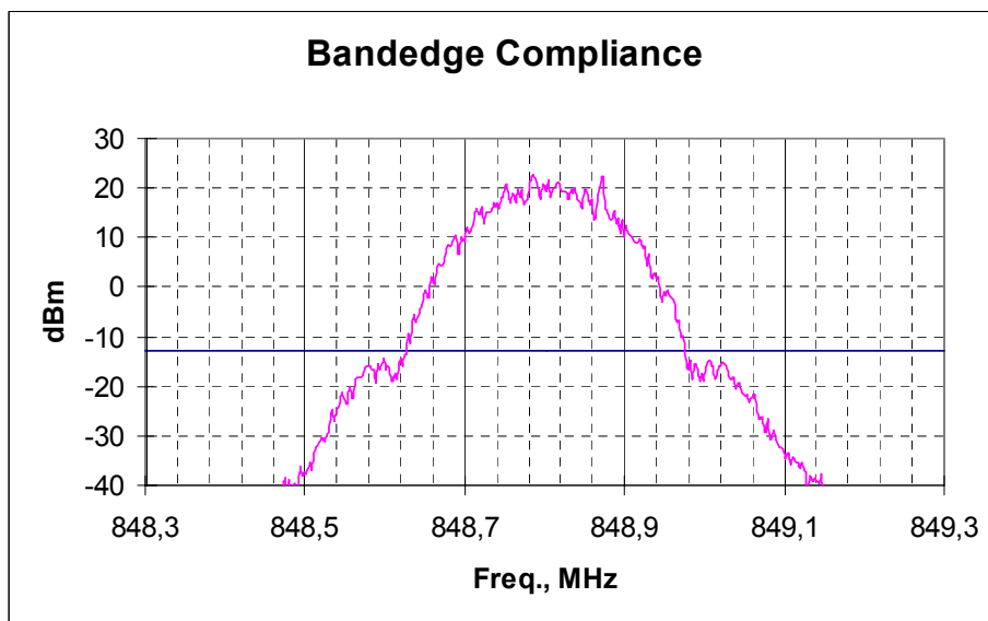
Picture 6. Upper bandedge, channel 251 RBw 3KHz VBw 3KHz
