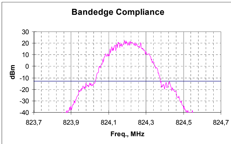
Picture 5. Lower bandedge, channel 128 RBw 3KHz, VBw 3KHz
