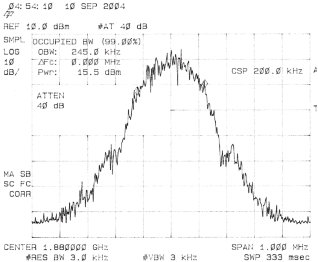
Picture 4. 99% occupied bandwidth, channel 661
