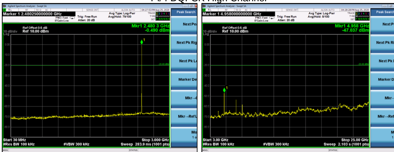
Pi/4 DQPSK High Channel
