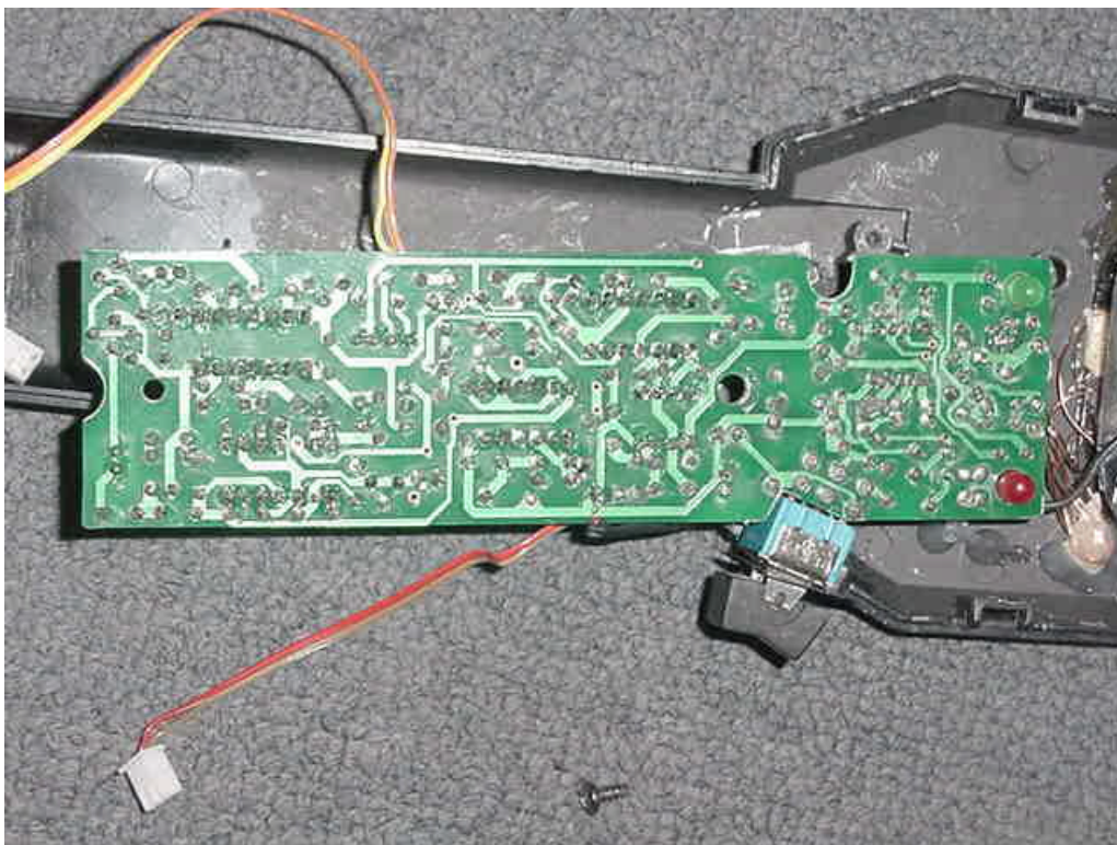
Soldered side
