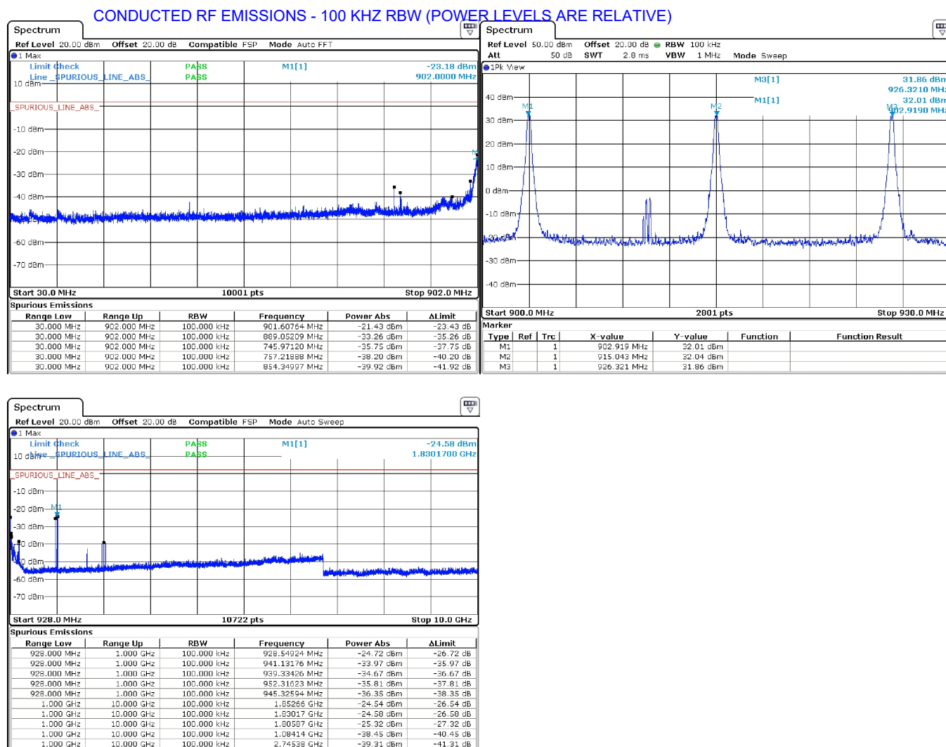
Figure 11: Conducted Transmitter Emissions Measured.
