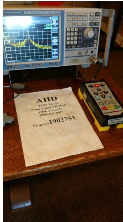
Figure 5: Conducted RF Test Setup Photograph(s).
