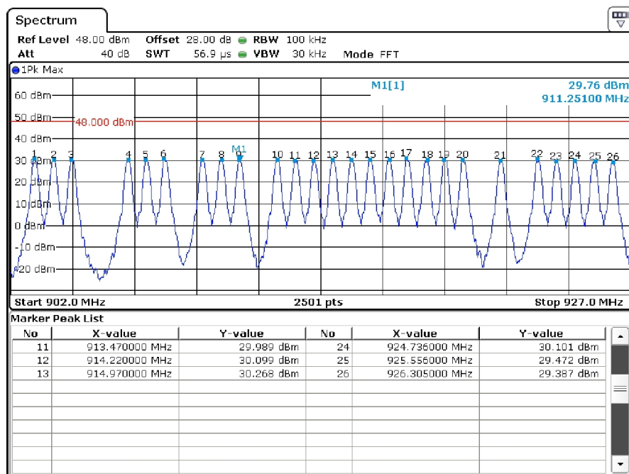
Figure 8: Measured Number of Hopping Channels.
