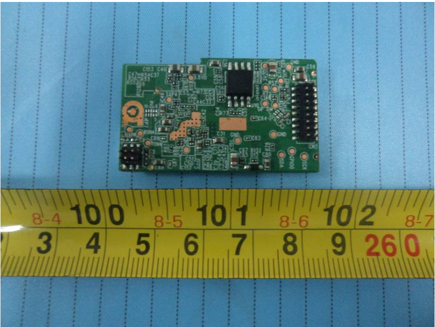
EUT – Wi-Fi Board Front View
