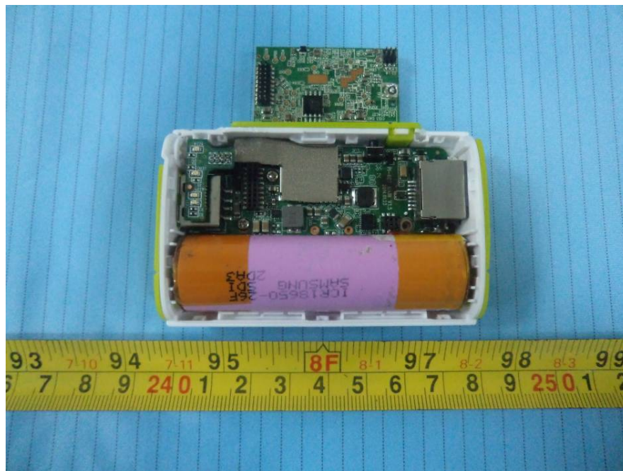
EUT – Cover off View 2 (Model: PON-WIFI-D11U-C26-WG)
