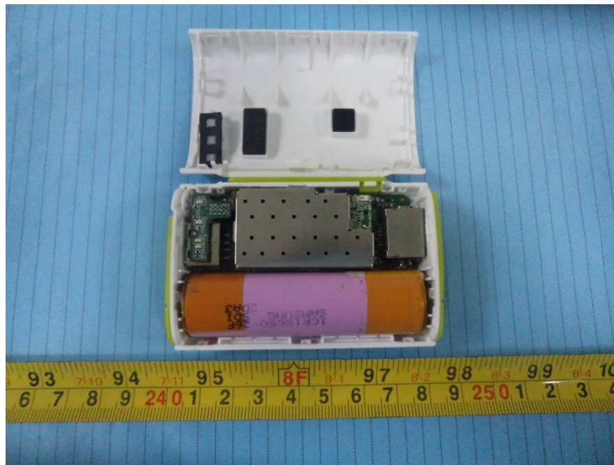
EUT – Cover off View 1 (Model: PON-WIFI-D11U-C26-WG)
