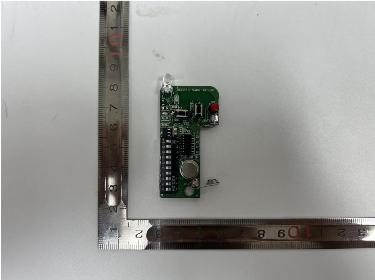
Front board
