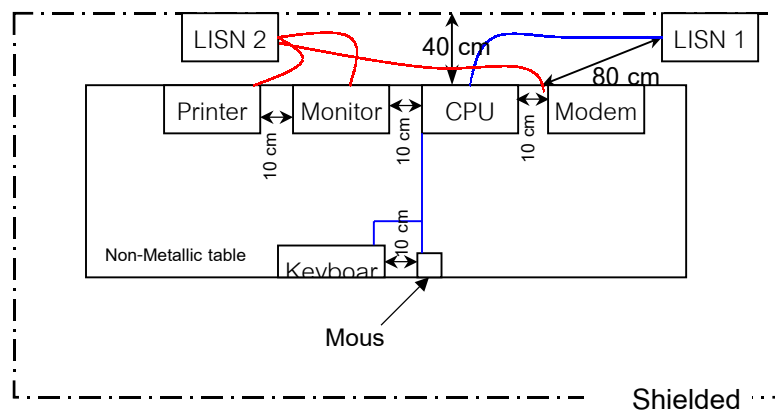
FIGURE 2. THE DIAGRAM OF SETUP FOR CONDUCTED EMISSIONS TESTING
