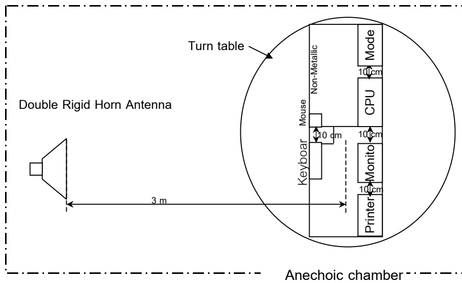
FIGURE 6. THE DIAGRAM OF SETUP FOR RADIATED EMISSIONS TESTING
