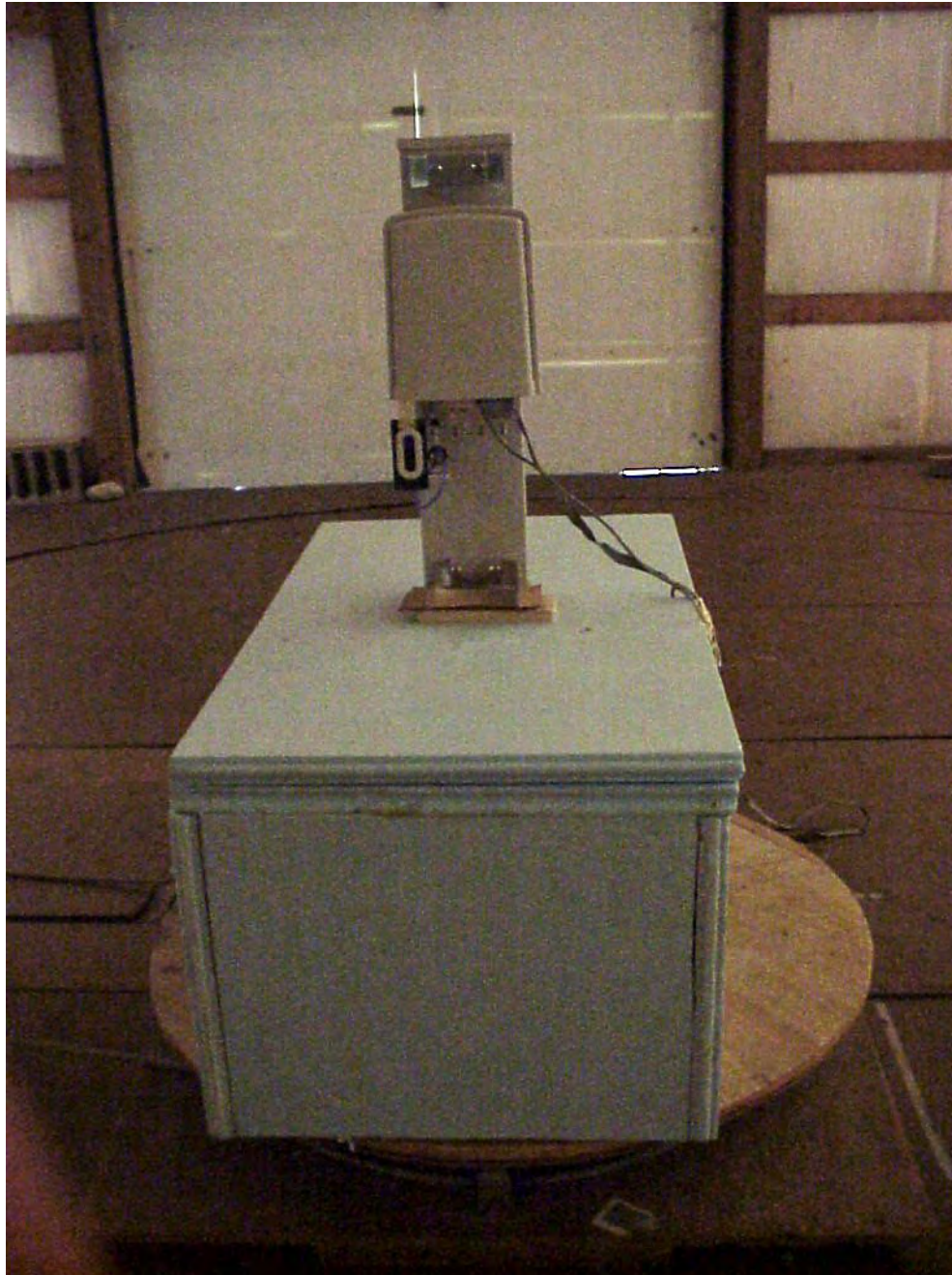
Radiated Side
