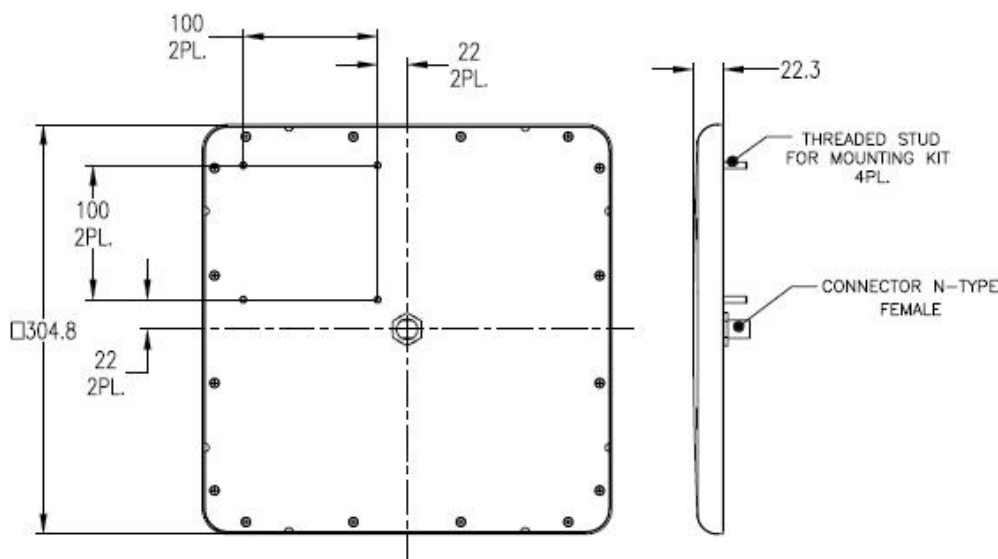
Dimensions [mm]
