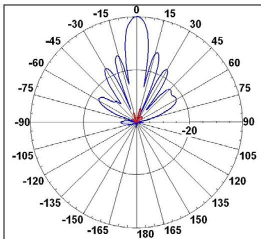
Elevation Radiation Pattern Midband Freq. 5.35 GHz
