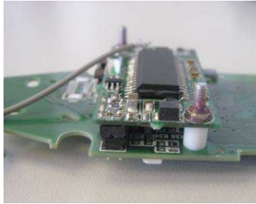
RFID decoder board
