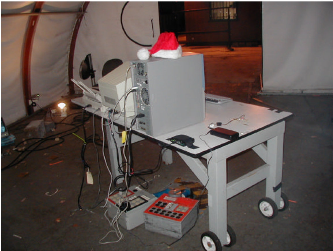
Radiated Emission Photo 2 of 2
