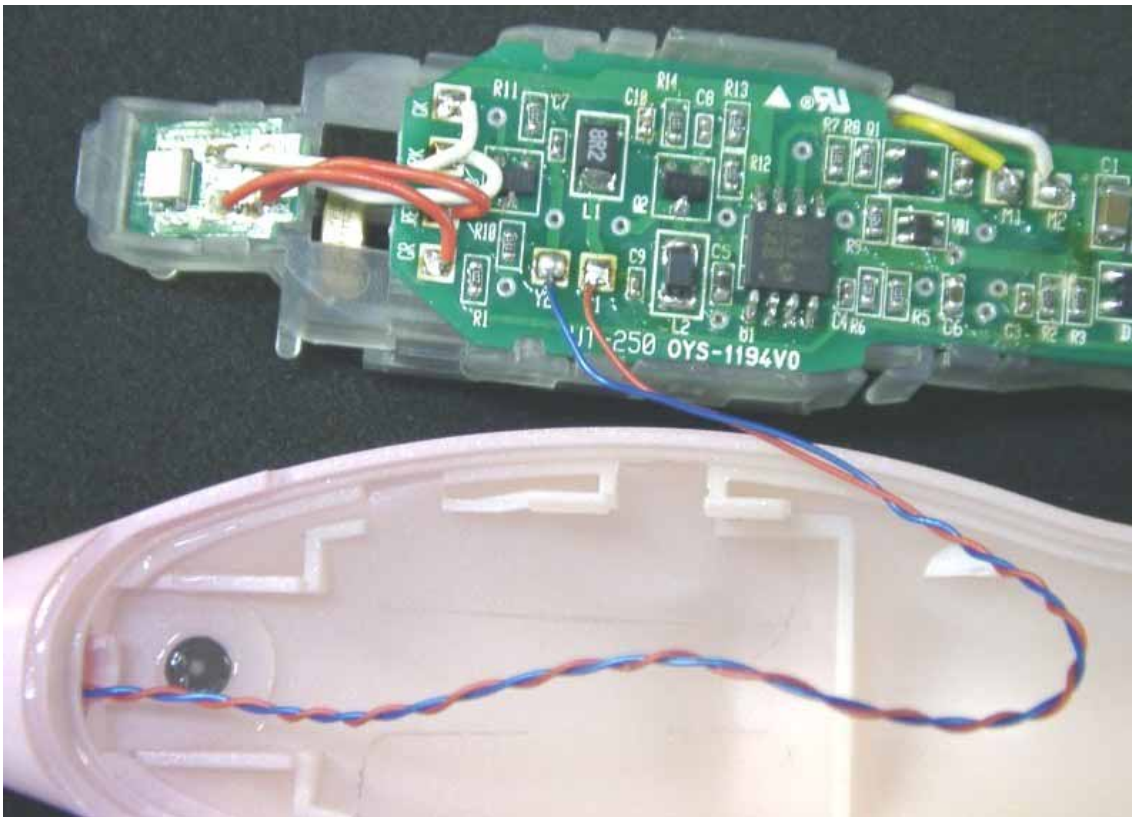
Internal Photo 2: Zoom-up inside of the tooth brush
