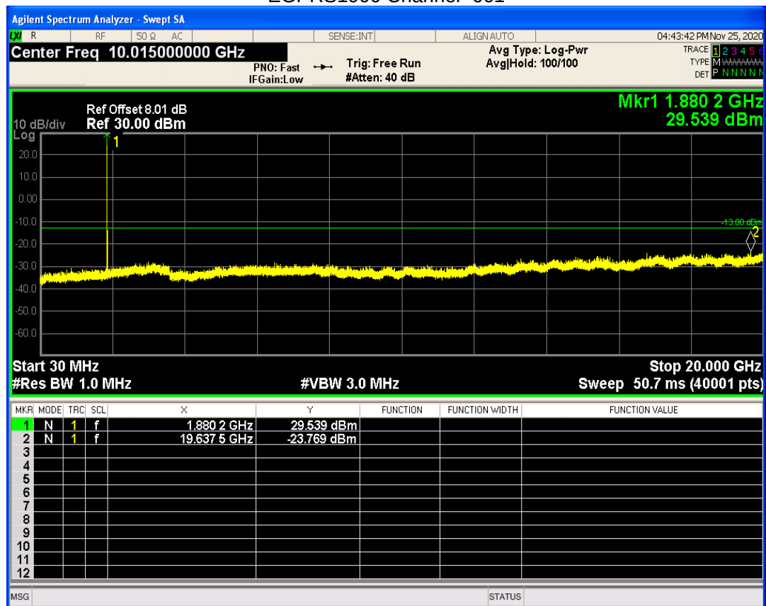
EGPRS1900 Channel=661
