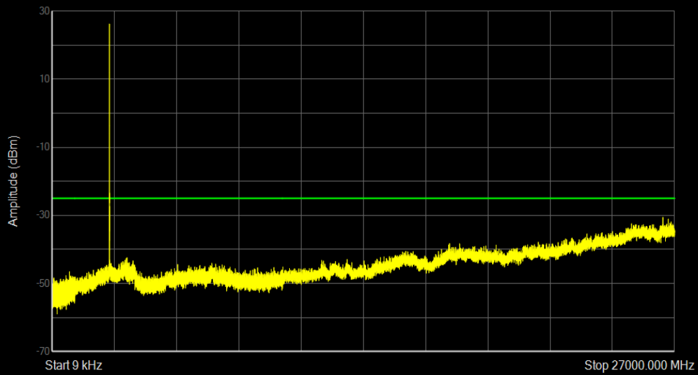
Band7 QPSK BW=5MHz Channel=20775 RB Size=1 Position=#0
