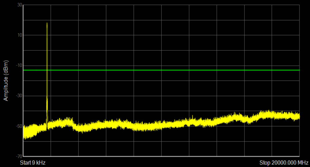
Band66 QPSK BW=15MHz Channel=132322 RB Size=75 Position=#0
