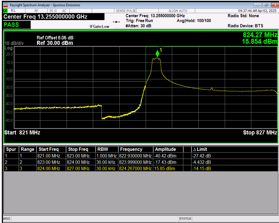
Band5 64QAM BW=3MHz Channel=20415 RB Size=1 Position=#Max
