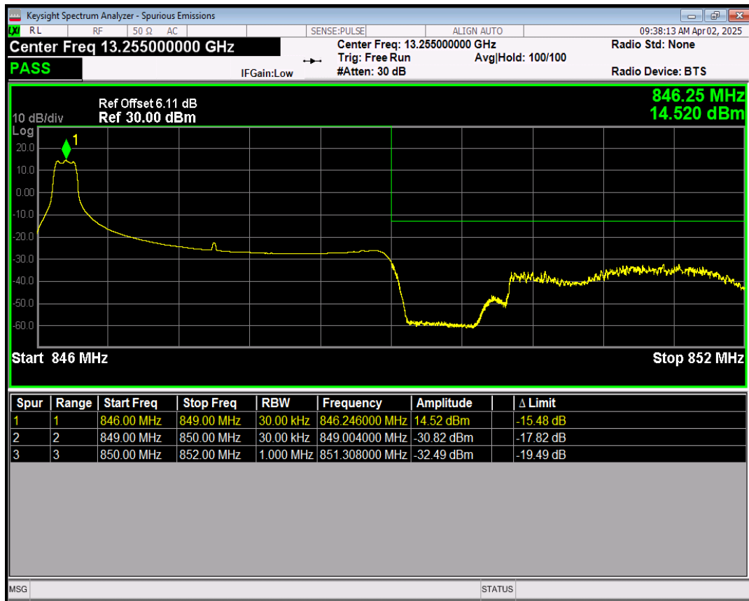
Band5 64QAM BW=3MHz Channel=20635 RB Size=1 Position=#Max
