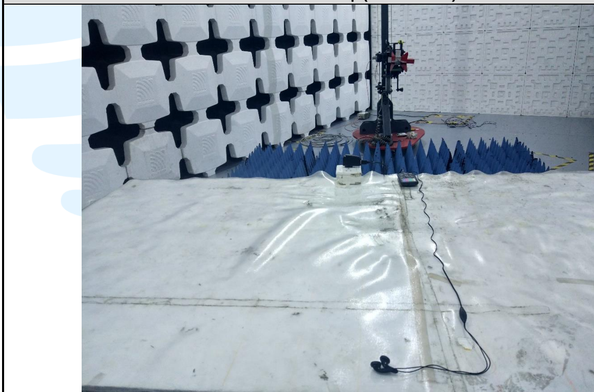
Radiated emission Test Setup (Above 1 GHz) – Mode3
