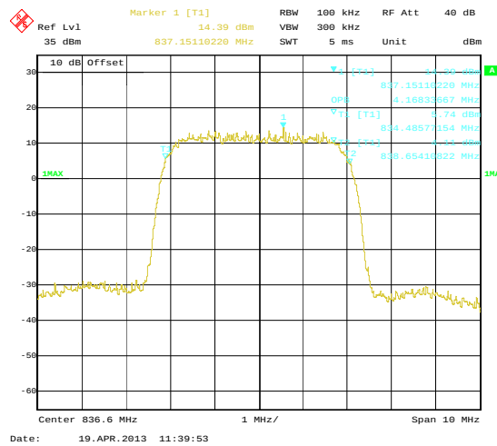
Middle channel
