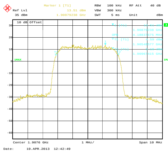
Highest channel
