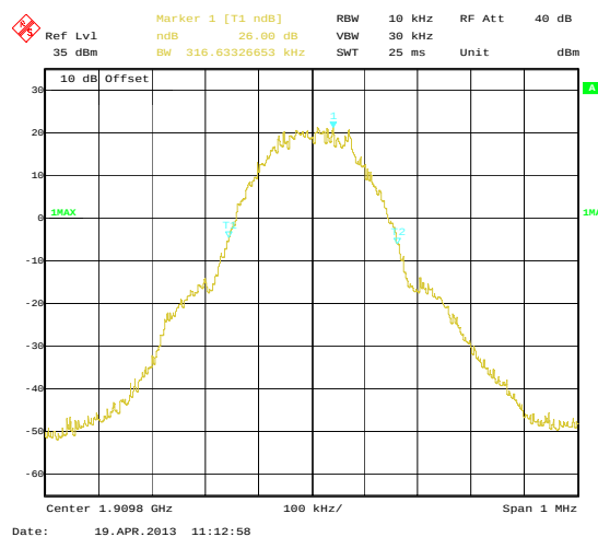
Highest channel
