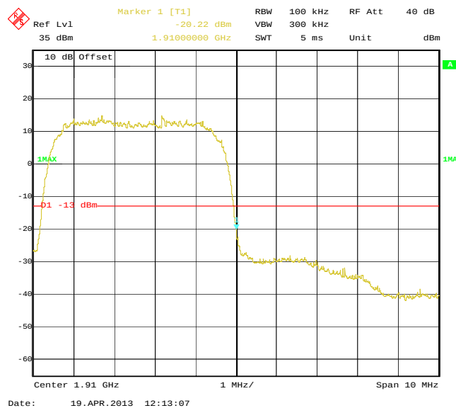
Highest channel
