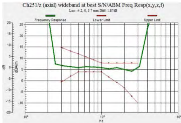
Fig 7.3 GSM850 Ch251
