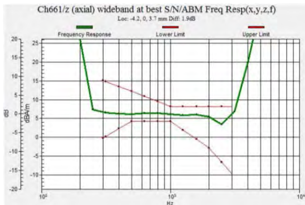
Fig 7.5 GSM1900 Ch661
