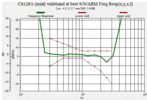
Fig 7.1 GSM850 Ch128
