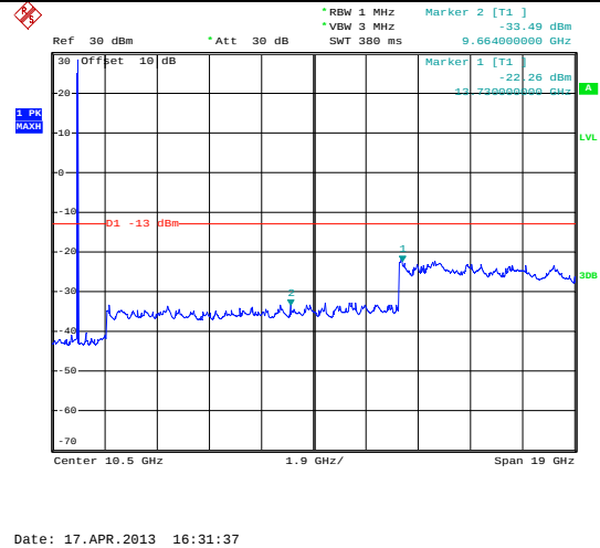
1GHz~20GHz
