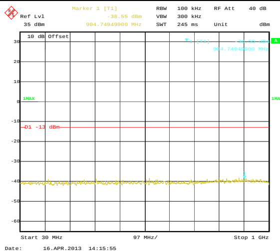
30MHz~1GHz
