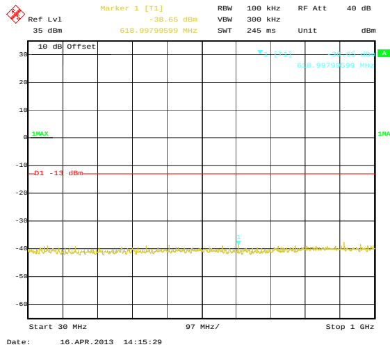
30MHz~1GHz
