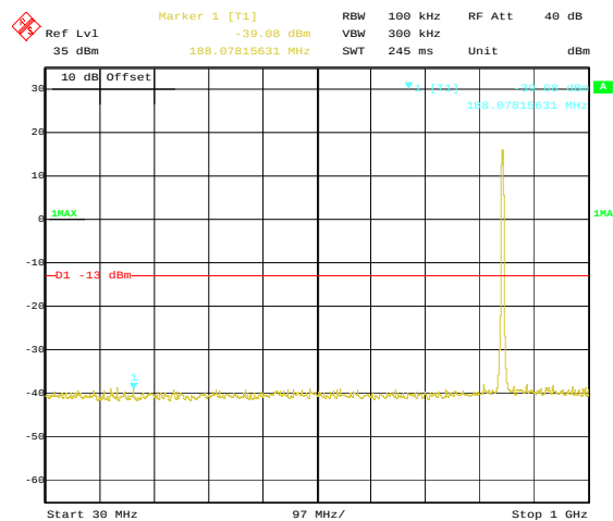
30MHz~1GHz
