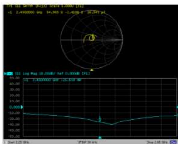
2450MHz Head
