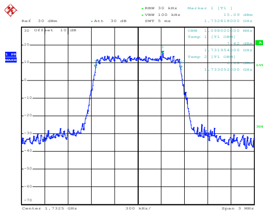
Modulation:16QAM
