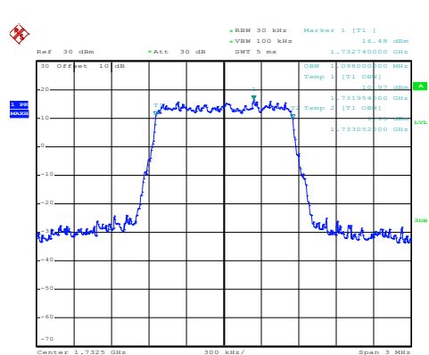
Modulation: QPSK
