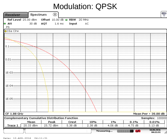
LTE Band 2 Middle channel
