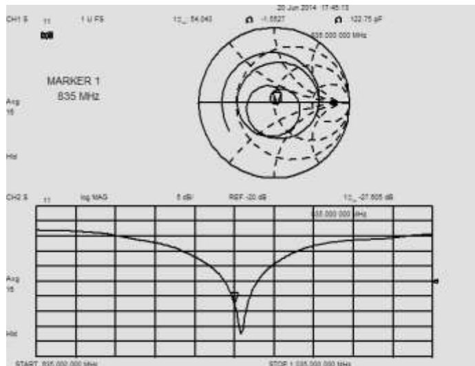
Measurement Plot for Head TSL In 2014
