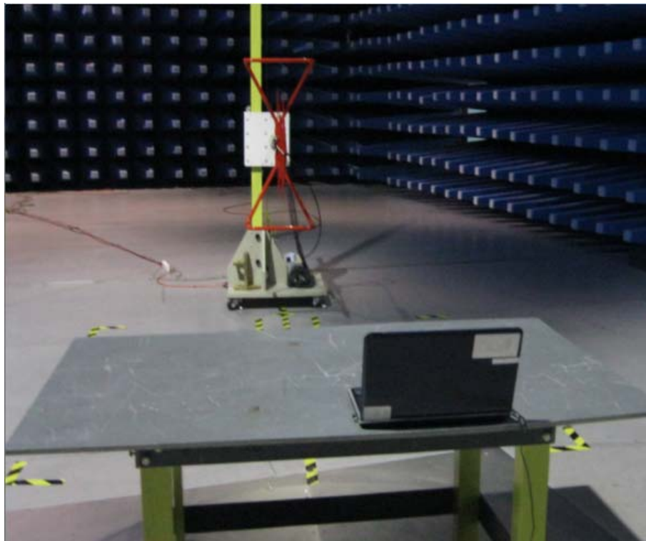
Radiated Spurious Emissions Test Setup Below 1GHz - Front View
