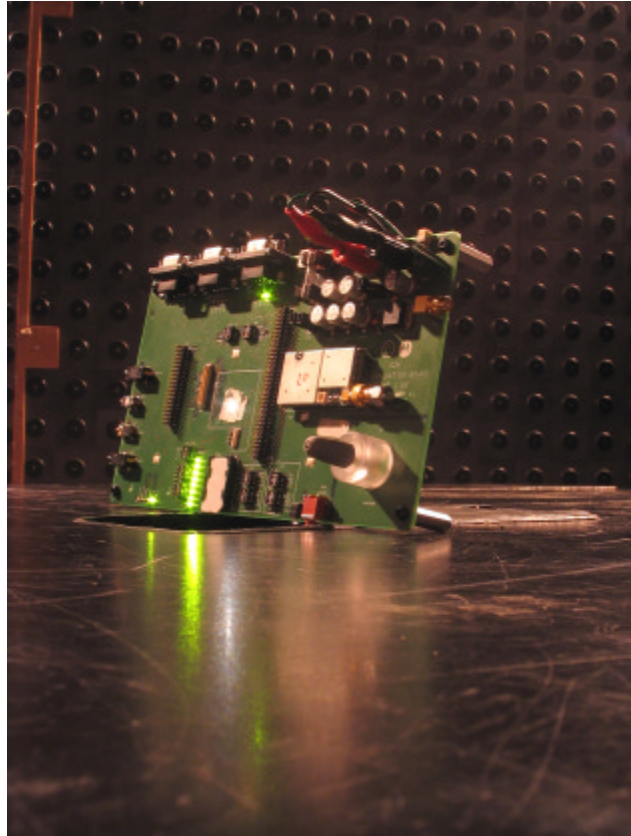
Photograph No.5 Radiated emissions measurement setup in the anechoic chamber EUT close view
