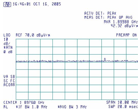
Plot 7.4.22 Radiated emission measurements at the third harmonic of low carrier frequency
