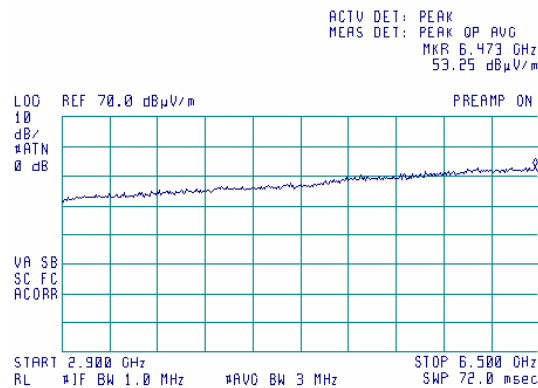
Plot 8.4.14 Radiated emission measurements from 2900 to 6500 MHz at the mid carrier frequency
