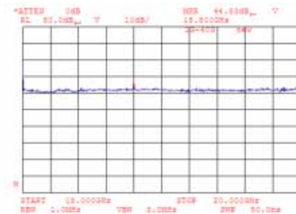
Plot 8.4.24 Radiated emission measurements from 18 to 20 GHz at the high carrier frequency
