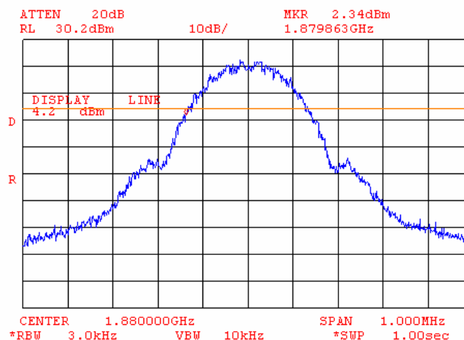
Plot 8.2.5 Occupied bandwidth test result at mid frequency, lower reference point
