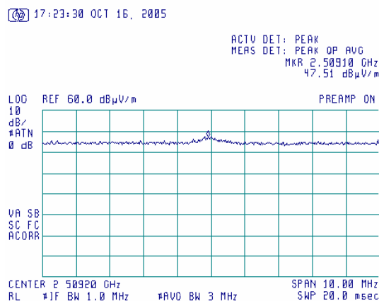
Plot 7.4.24 Radiated emission measurements at the third harmonic of high carrier frequency
