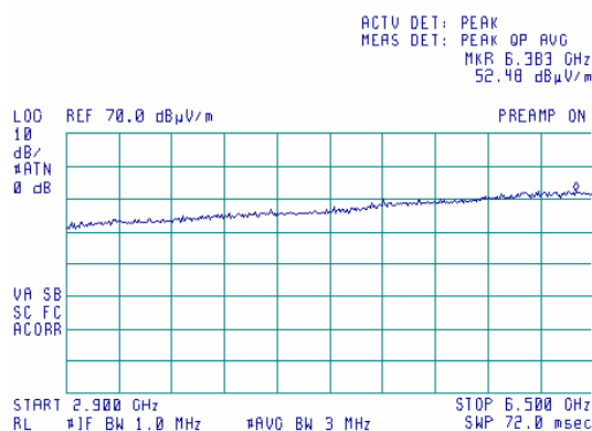
Plot 7.4.14 Radiated emission measurements from 2900 to 6500 MHz at the mid carrier frequency
