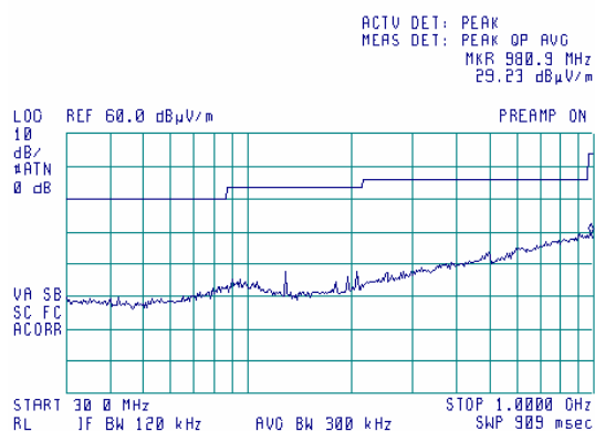
Plot 8.4.8 Radiated emission measurements from 30 to 1000 MHz at the mid carrier frequency
