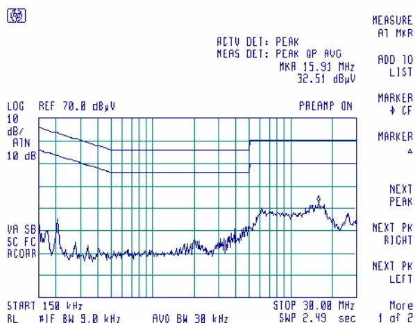
Plot 9.1.2 Conducted emission measurements
