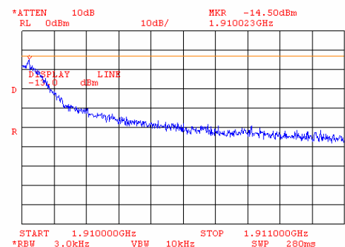
Plot 8.2.11 Bandedge emission measurements in 1910 - 1911 MHz range at high carrier frequency
