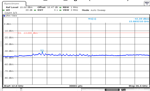
GPRS_1900_Higher(12GHz-26.5GHz)
