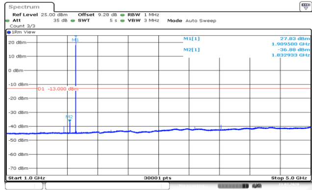
GPRS_1900_Higher(1GHz-5GHz)
