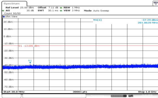
GPRS_1900_Higher(30MHz-1GHz)
