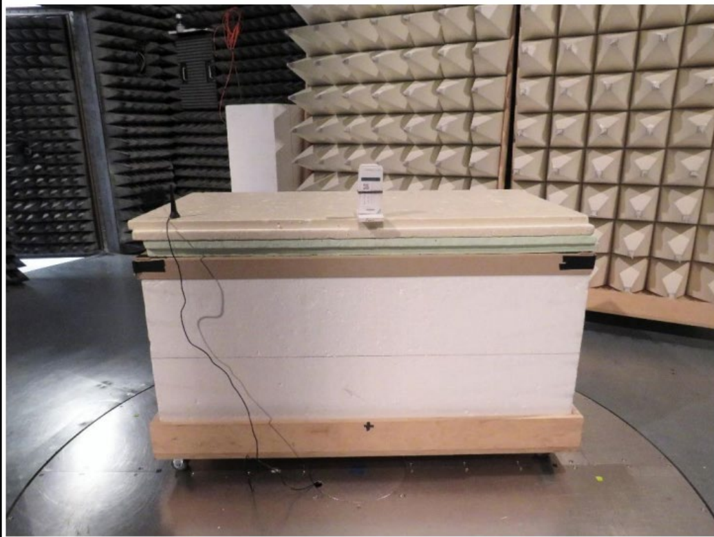
EUT Setup radiated emissions below 1 GHz
