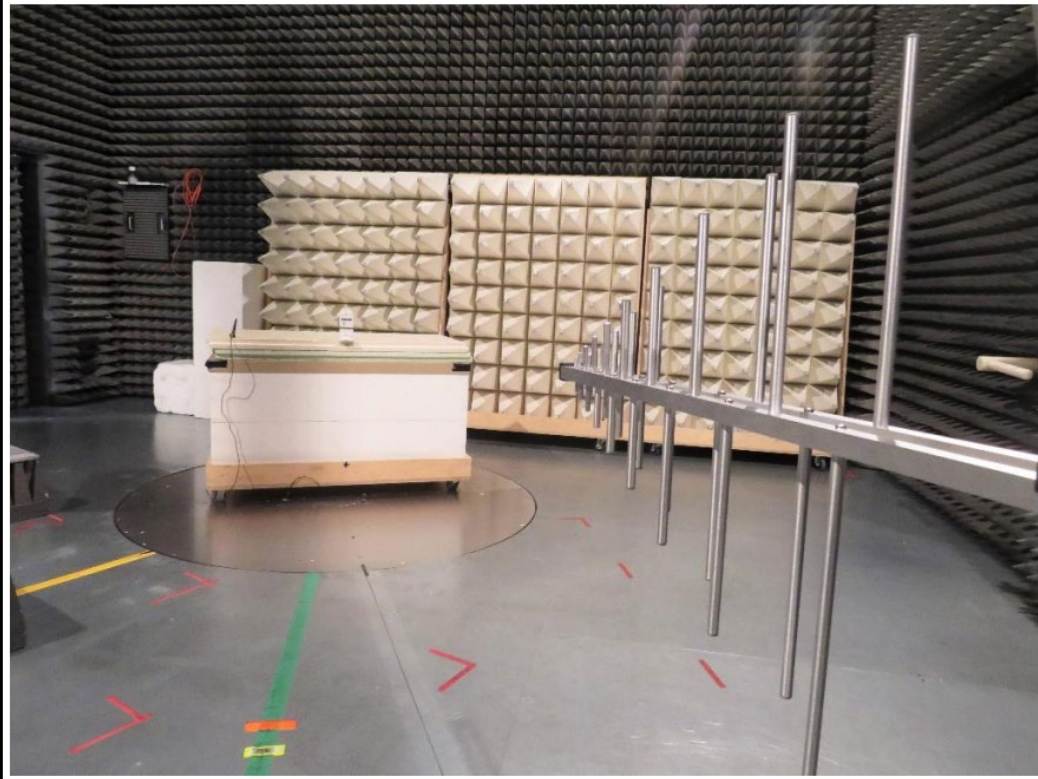
Test Setup radiated emissions below 1 GHz
