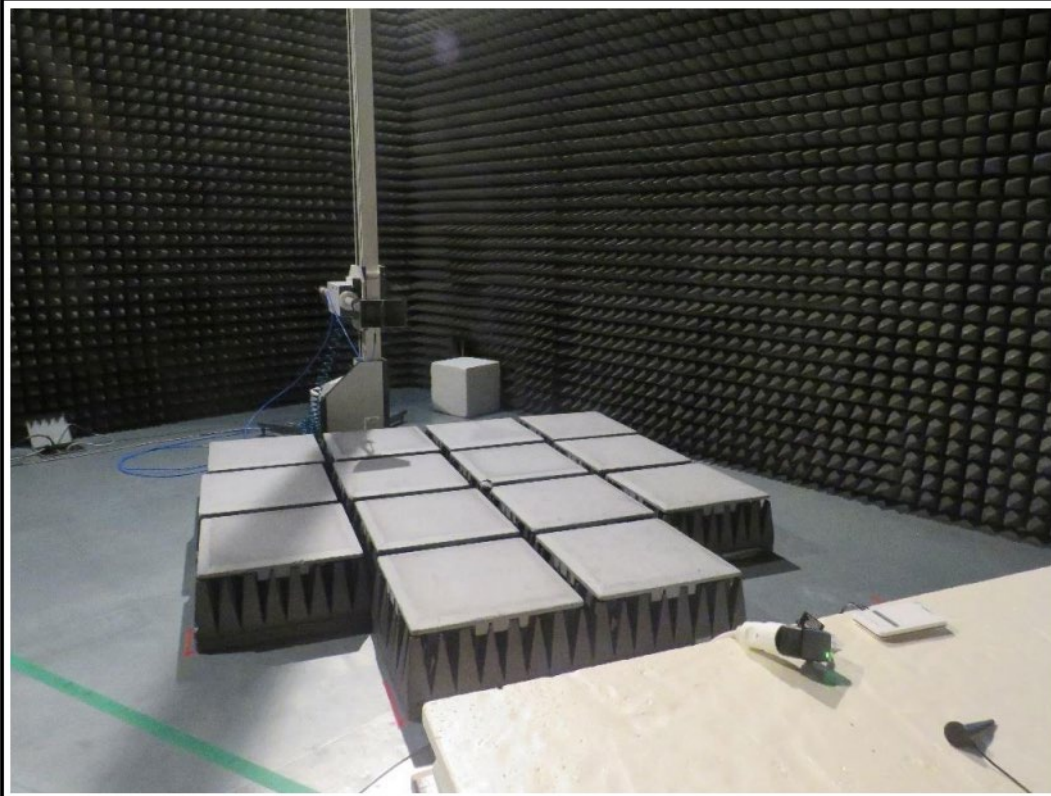
TEST SETUP – 1 GHz to 11 GHz - CONFIGURATION 1
