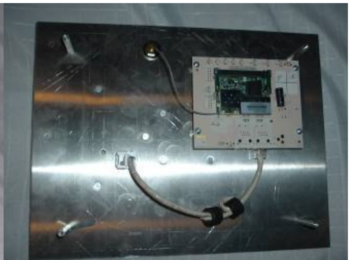
Figure 8 – Carrier/radio mounted to backplate
