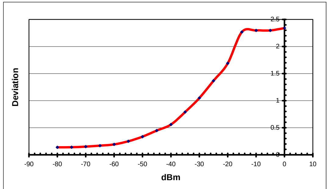
MODULATION LIMITING PLOT - 300 Hz
