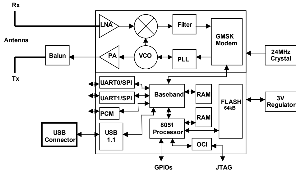
MT0760-UD-2 Module Block Diagram
