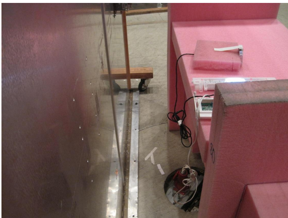
Photo 4.1.2 Test setup regarding measurement of conducted limits, AC Mains.
