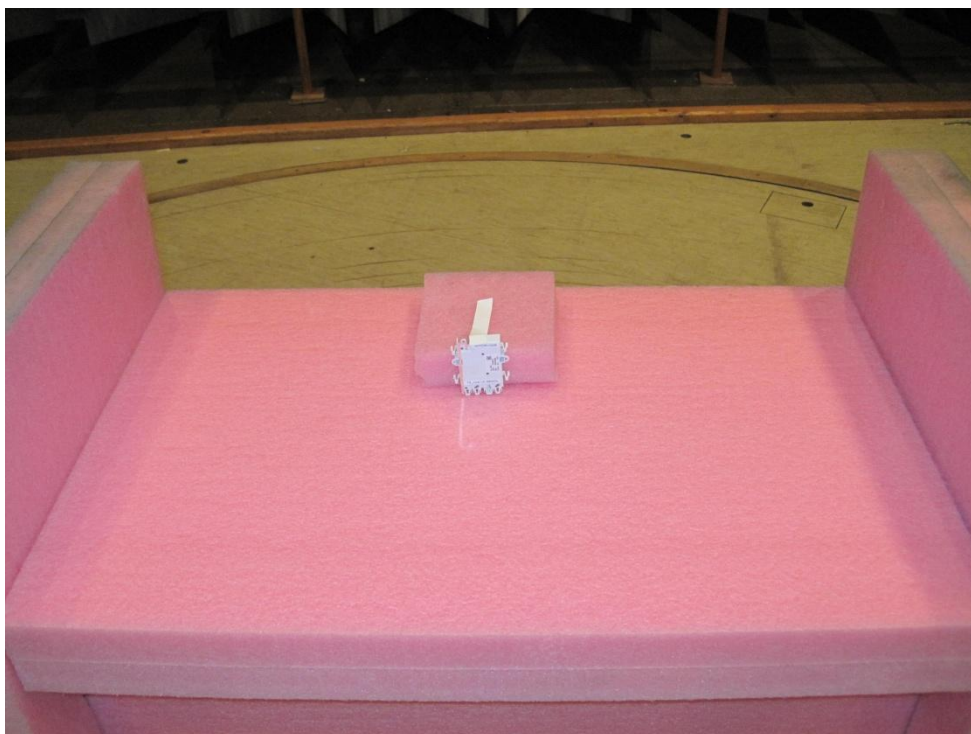
Photo 4.2.2 Test setup regarding measurement of radiated limits below 1 GHz.
