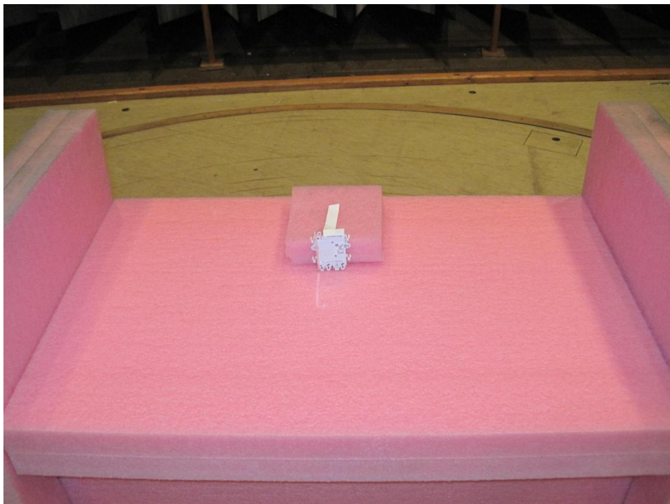
Photo Error! No text of specified style in document. 8.2 Test setup regarding measurement of field strength of the fundamental.
