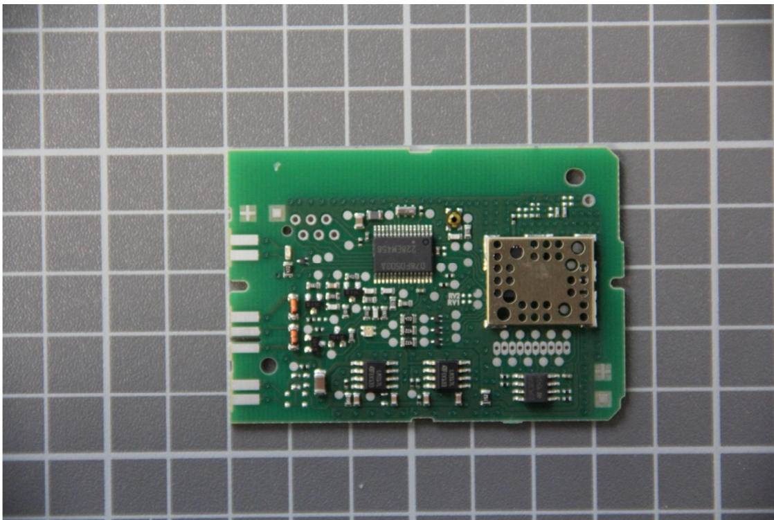
Pic. 1 assembled PCB (bottom side)
