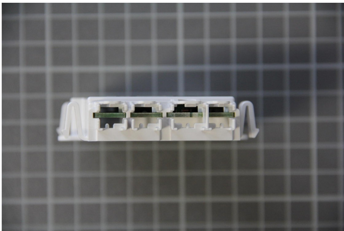
Pic. 9 Housing with assembled PCB (side view, connector)
