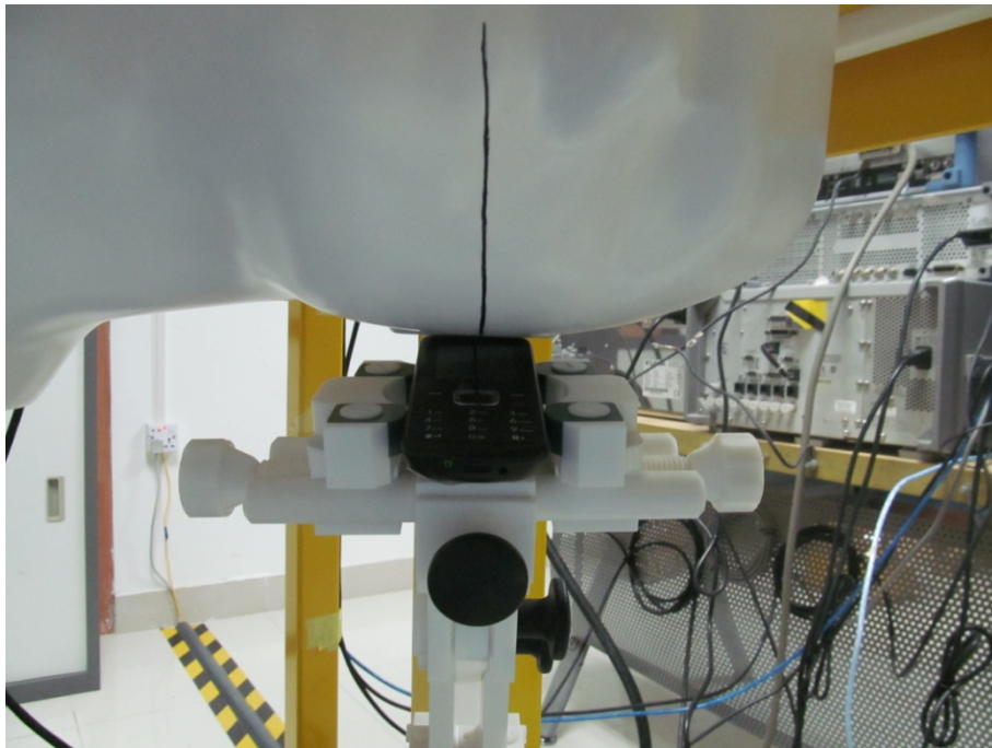
LEFT-TILT 15^{\circ}
