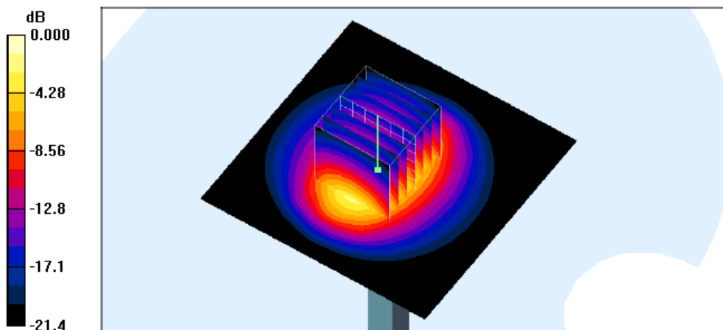
0 dB = 6.05mW/g
