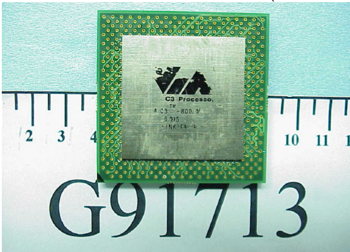
Figure 18 CPU (VIA C3 800 MHz)
