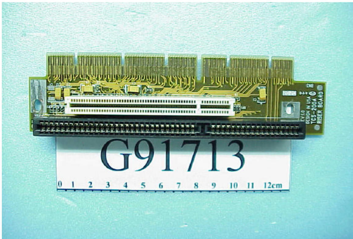
Figure 10 RISER Board
