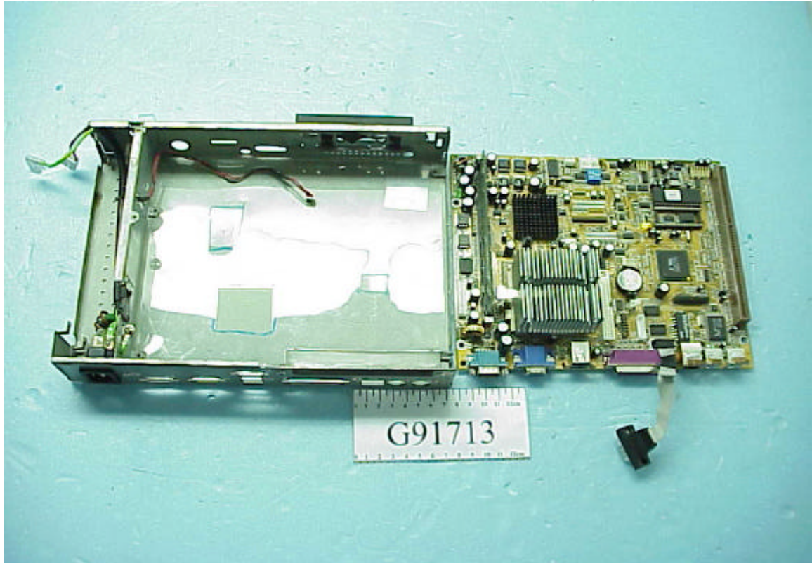
Figure 15 Internal View (Remove Main Board)
