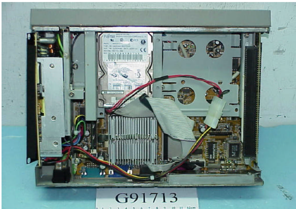
Figure 6 Internal View
