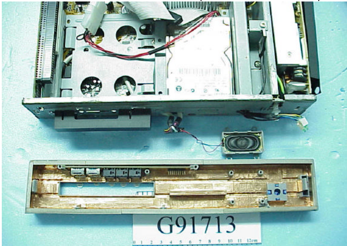
Figure 7 Internal View (Remove Front Panel & Speaker)
