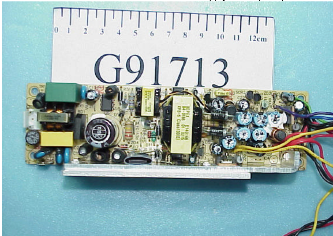
Figure 31 Power Supply- 25W (Component Side)
