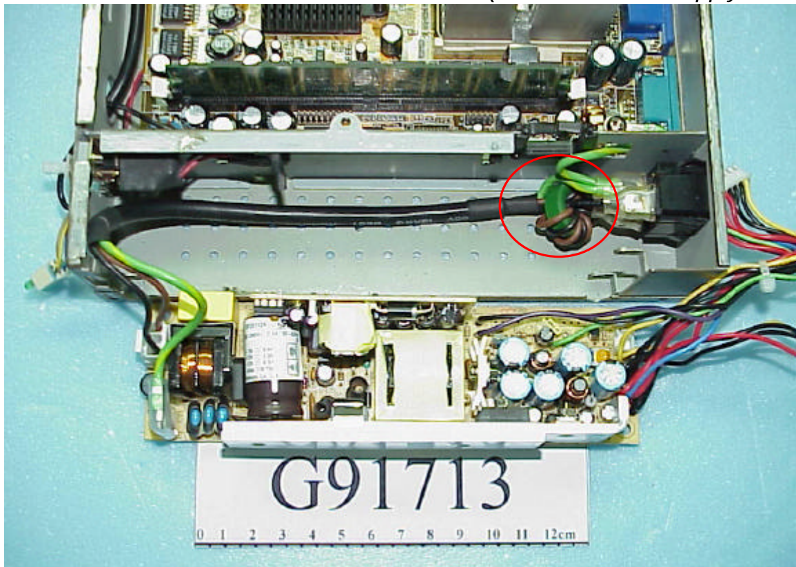
Figure 28 Internal View (Remove Power Supply- 60W)
