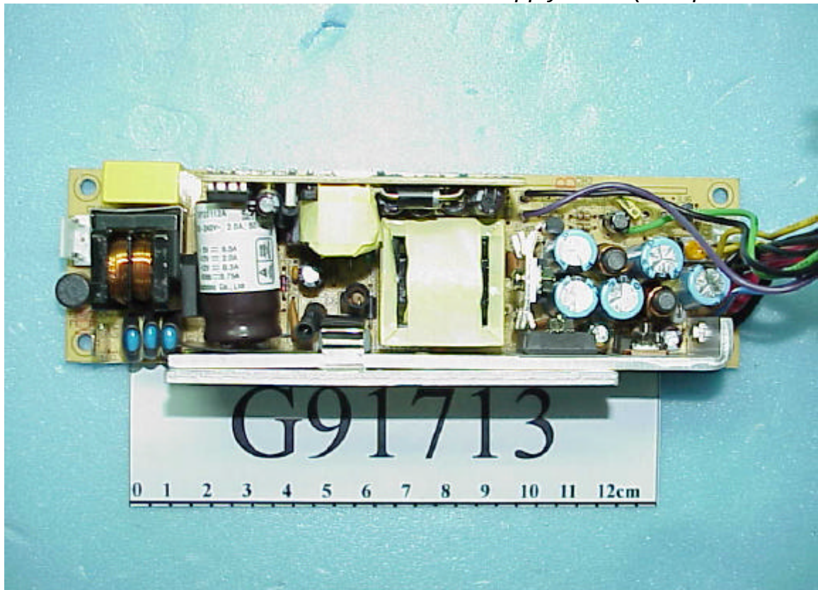
Figure 29 Power Supply- 60W (Component Side)
