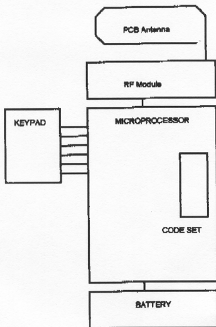
TRANSMITTER BLOCK DIAGRAM
