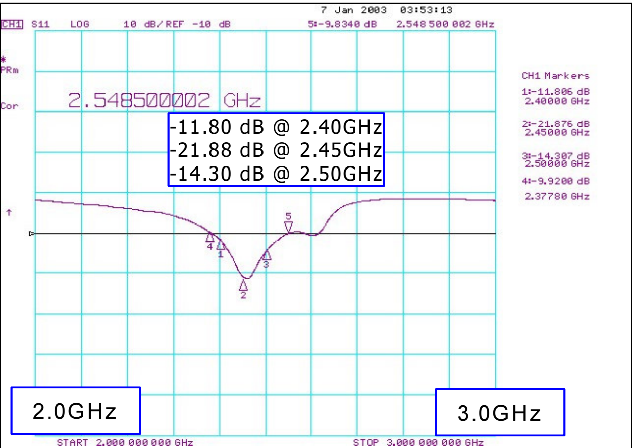
S11 for Antenna - 1:
