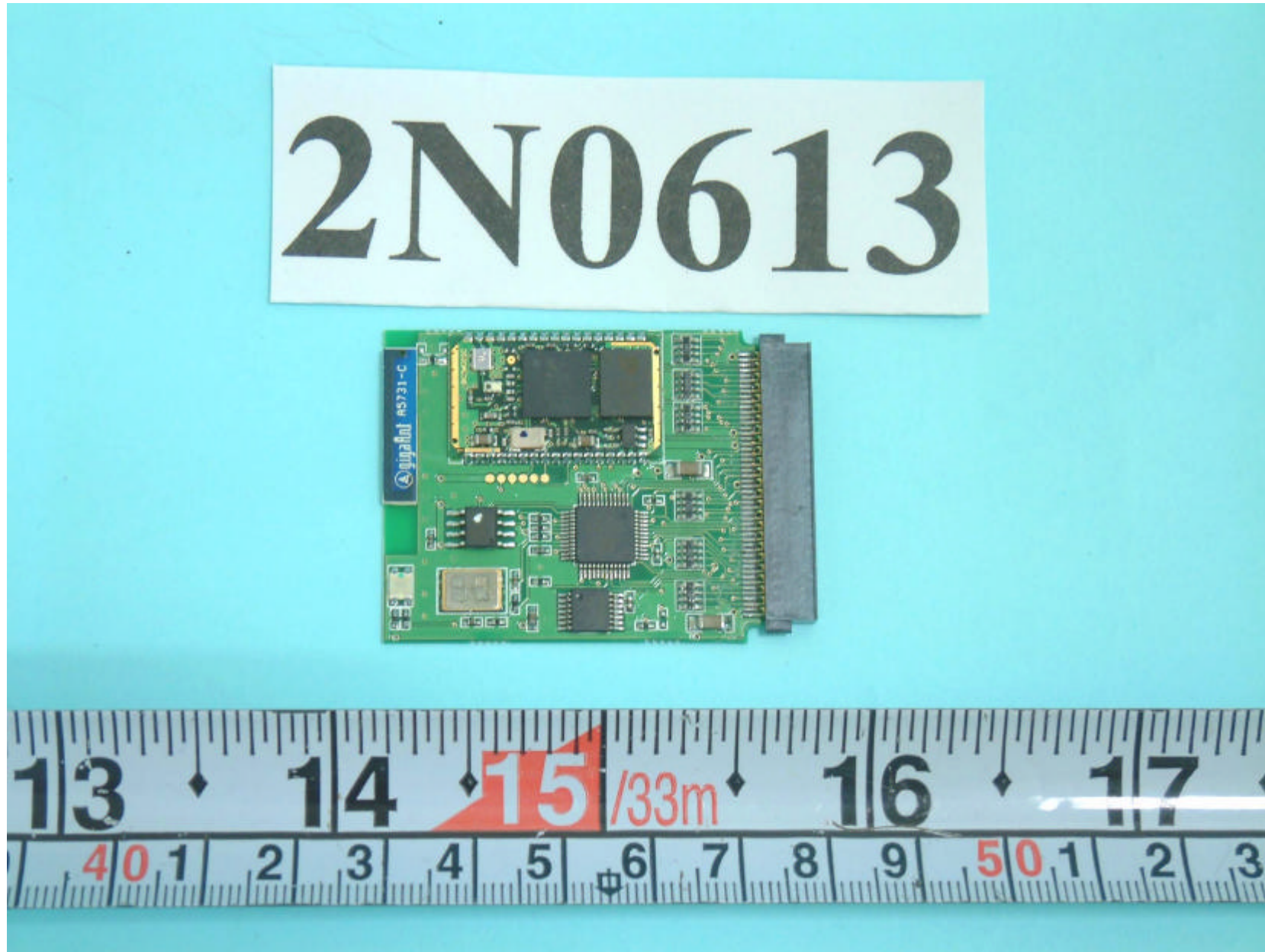
Front side of Main Board
