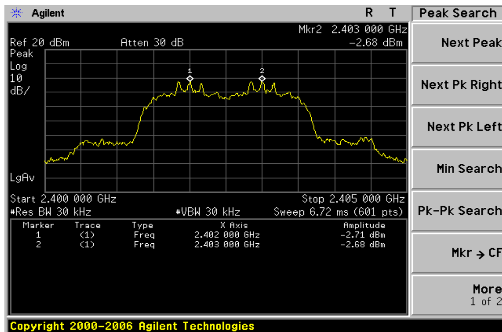
TEST PLOT FOR FREQUENCY SEPARATION (3Mbps)
