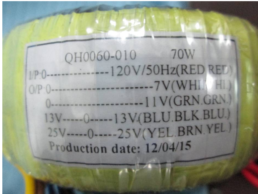
EUT – Coil View (Power supply)
