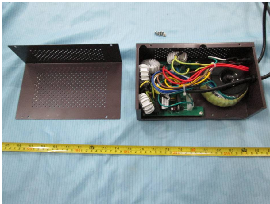
EUT –Cover off View (Power supply)
