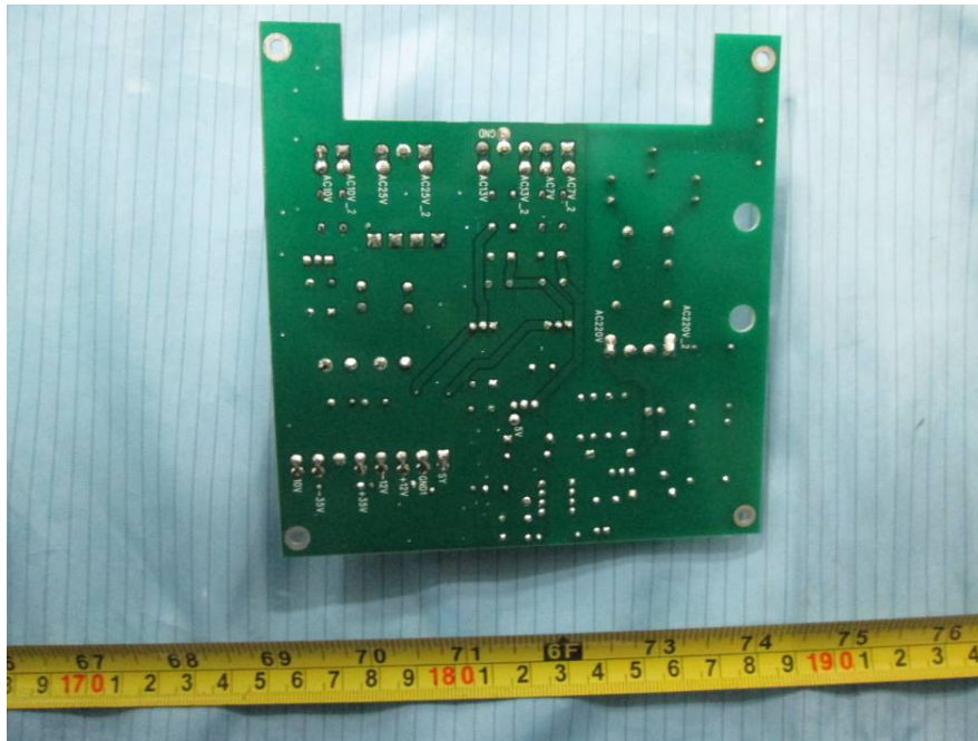
EUT – Main Board Bottom View (Power supply)
