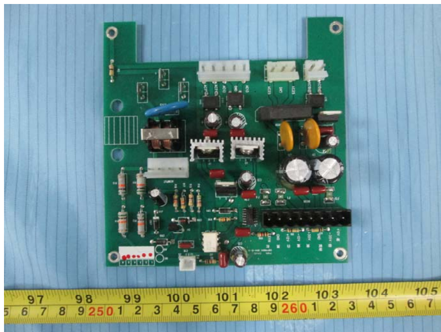
EUT – Main Board Top View (Power supply)
