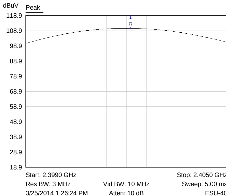
Lowest Channel Fundamental Field Strength
