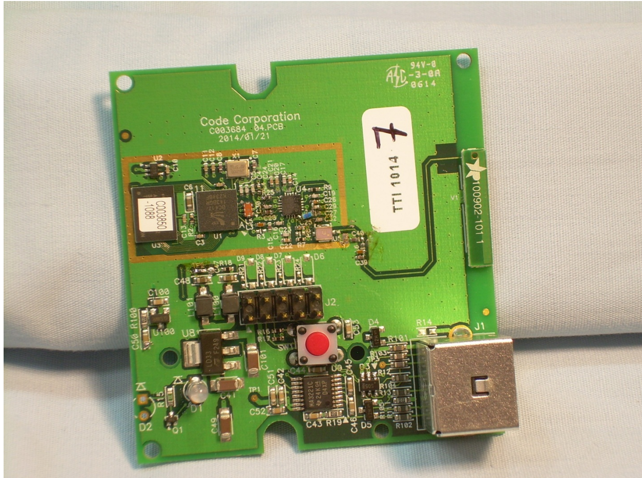
View of the Top Side of the PCB with RF Shield Removed
